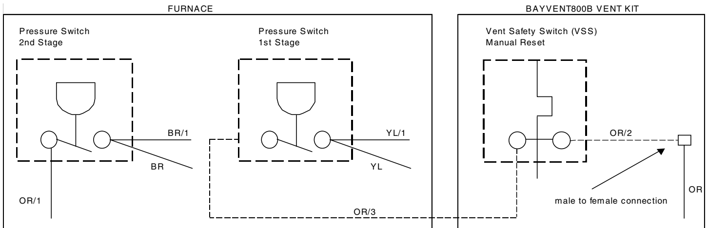
WIRING DIAGRAM 2 - TWO STAGE FURNACE
