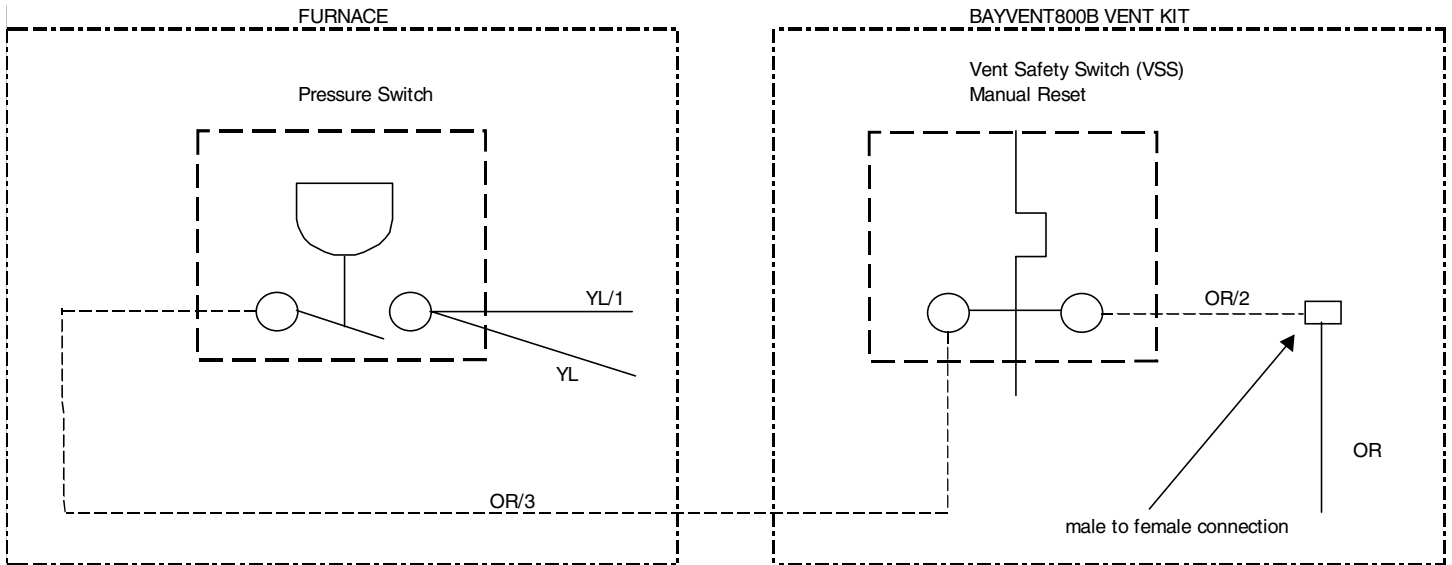
WIRING DIAGRAM 1 - SINGLE STAGE FURNACE
